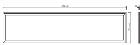
LD-GL40120
