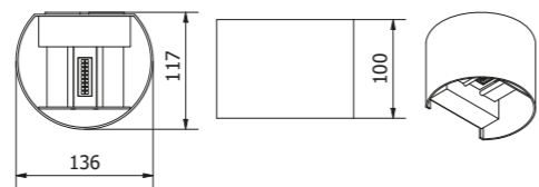
LD-MISS7WOC-NB LD-MISS7WOS-NB
