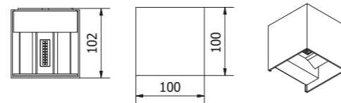
LD-MISS7WKC-NB LD-MISS7WKS-NB
