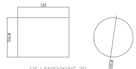
OS-LEN100KKG-30
